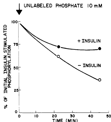
FIGURE 5: Pulse-chase of the ^{32}\text{PO}_4^{3-} incorporated into the \beta -subunit of the insulin receptor from Fao cells. Fao cells were labeled at 37^\circ\text{C} for 2 h with ^{32}\text{PO}_4^{3-} and then incubated in the same medium for an additional 30 min in the presence of insulin ( 10^{-7} M). A cell sample was also incubated in the absence of insulin for 30 min to provide a measure of the basal phosphorylation. After this time interval, the basal phosphorylation reaction and one insulin stimulated reaction were stopped. The radioactive incubation media were removed from the other insulin-stimulated cells and replaced by a medium containing 10 mM unlabeled phosphate and either 10^{-7} M insulin ( \bullet ) or no insulin ( \circ ). These reactions were stopped after the time intervals indicated on the abscissa, the insulin receptor was purified and immunoprecipitated, and the proteins were separated by SDS-PAGE under reducing conditions. The labeling of the \beta -subunit was quantified by scanning densitometry of autoradiograms. The basal phosphorylation was deducted from the amount of phosphorylation found after 30 min of insulin stimulation only, and this value was taken as 100%. The values found after addition of unlabeled phosphate in the presence (+) and absence (-) of insulin were also corrected for the basal phosphorylation and are expressed as a percentage of the insulin effect before addition of unlabeled phosphate.
